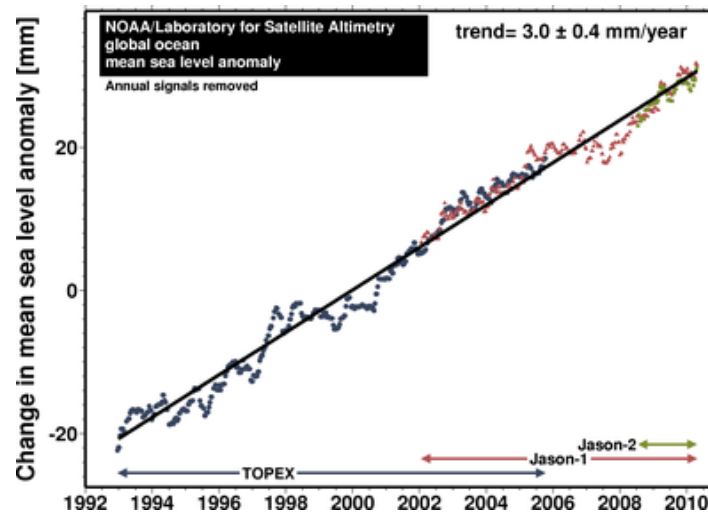
Figure 2.4. The estimated rate of global sea level rise since 1992 using satellite altimeter data.
