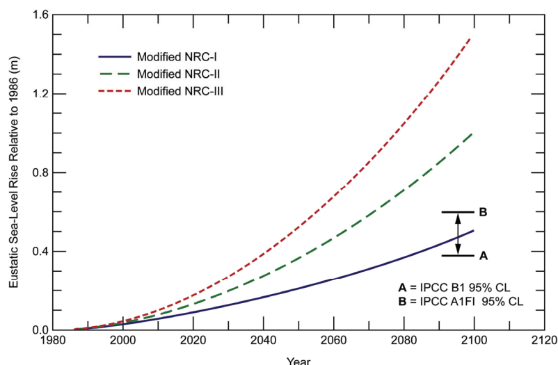
Figure 2.19. Taken from USACE (2009) comparing the modified NRC (1987) curves compared to the IPCC (2007) model results.
