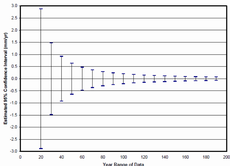
Figure 2.14. A 95% confidence interval for linear mean sea level trend versus series length (Zervas 2009).
