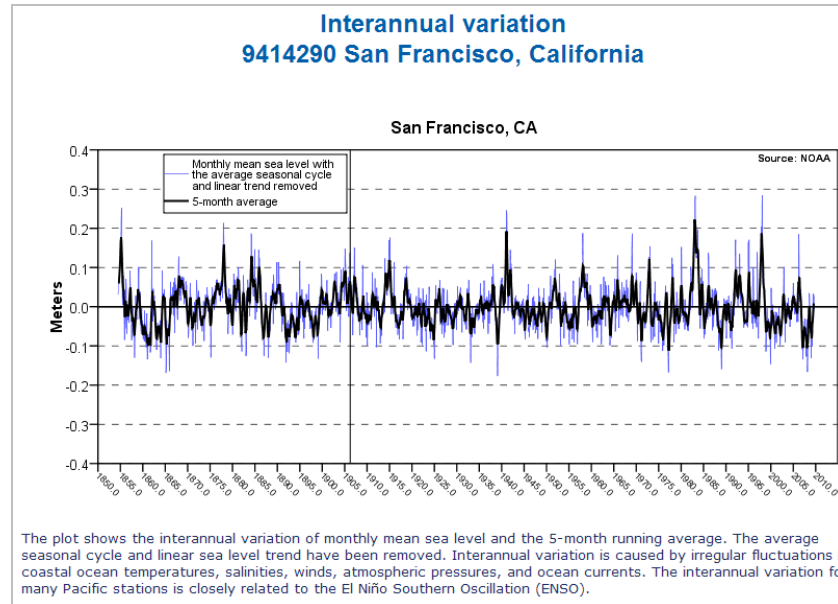
Figure 2.11. The interannual variation in monthly mean sea level at San Francisco
