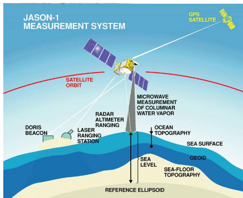
Figure 3.5. Schematic of a satellite altimeter configuration.
